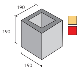
Half Hollow 190 x 190 x 190mm 9kg. 3MPa (5N/mm 2 )
