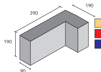
Quoin/Cavity Closer 390 x 190 x 90/190mm 17kg. 5MPa (5N/mm 2 )
