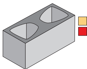
Hollow 390 x 190 x 190mm 18kg. 3MPa (3N/mm 2 )
