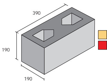
Hollow (25% Void) 390 x 190 x 190mm 25kg. 5MPa (5N/mm 2 )
