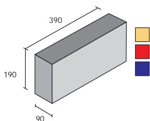
Solid 390 x 190 x 90mm 13kg. 5MPa (5N/mm 2 )
