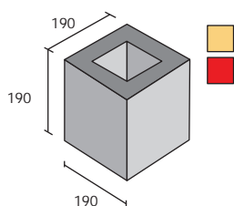
Half Hollow (25% Void) 190 x 190 x 190mm 13kg. 5MPa (5N/mm 2 )
