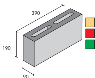
Hollow 390 x 190 x 90mm 11kg. 5MPa (5N/mm 2 )
