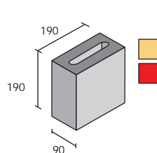
Half Hollow 190 x 190 x 90mm 6kg. 5MPa (5N/mm 2 )
